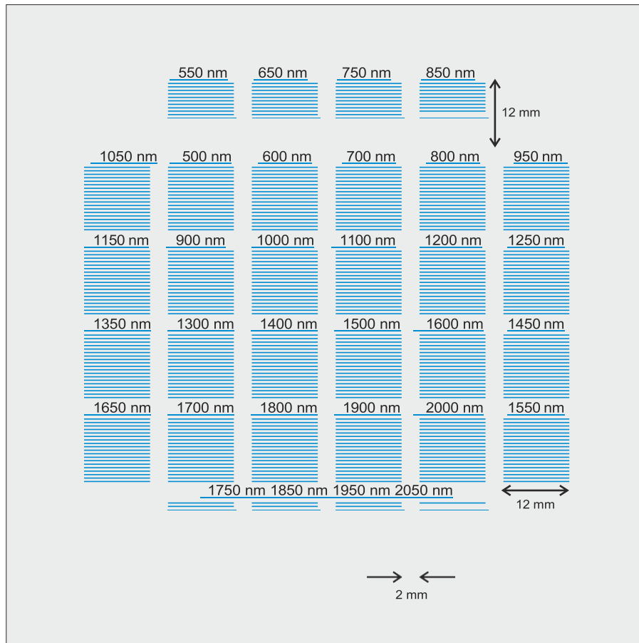
Layout of MP500L2050 drawing not to scale
